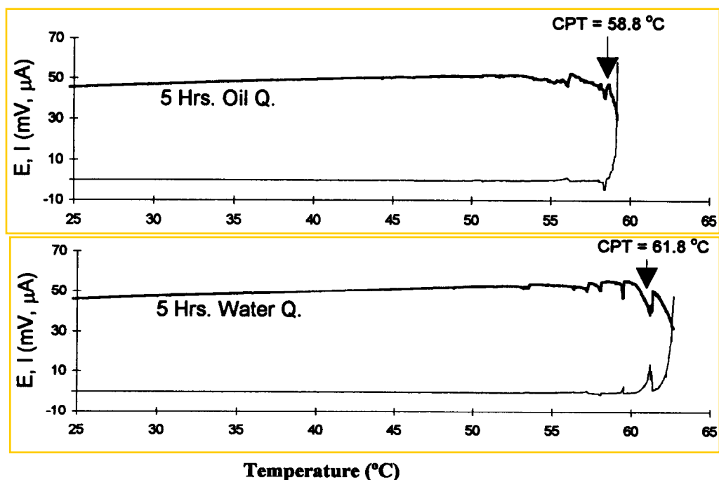
Fig. 2. The critical pitting temperature of alloy UNS S32550 annealed at 1060°C and quenched under the conditions indicated, determined by using the ZRA test. (—) Potential (mV(SCE) \times 10); (---) current ( \mu\text{A} ).
